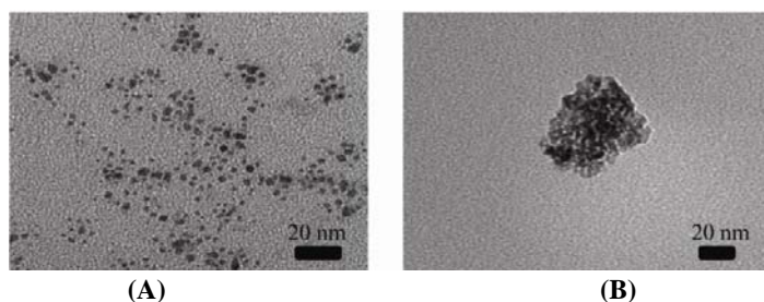
Figure 17. Transmission Electron Microscope (TEM) image of aerosol-generated \text{TiO}_2 nanoparticles. (A) Un-aggregated and (2-5 nm) (B) and aggregated (80-120 nm), used in exposure studies to determine the health impacts of manufactured nanoparticles. Nanoparticle aggregation may play an important role in health and environmental impacts. (Images courtesy of Vicki Grassian, University of Iowa [Grassian, et al., unpublished results])
