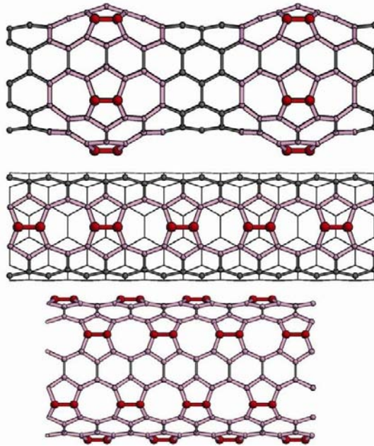
Figure 4. Computer images of various forms of carbon nanotubes. (Images courtesy of Center for Nanoscale Materials, (Images courtesy of Center for Nanoscale Materials, Argonne National Laboratory)
