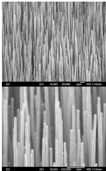
Figure 5. “Forest” of aligned carbon nanotubes. (Image courtesy David Carnahan of NanoLab, Inc.)
