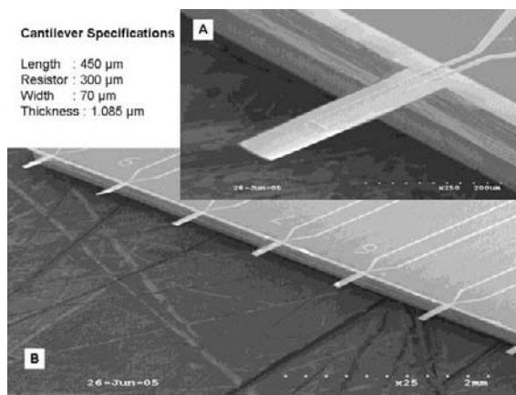
Figure 14. Piezoresistive cantilever sensor.
