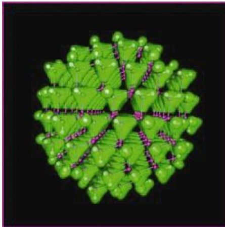
Figure 7. Computer image of a Gallium arsenide quantum dot of 465 atoms. (Image courtesy of Lin-Wang Wang, Lawrence Berkeley National Laboratory)
